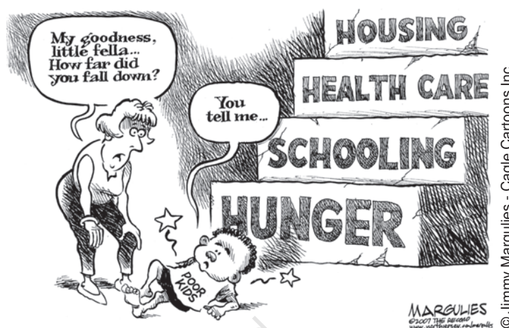
Poor Kids
