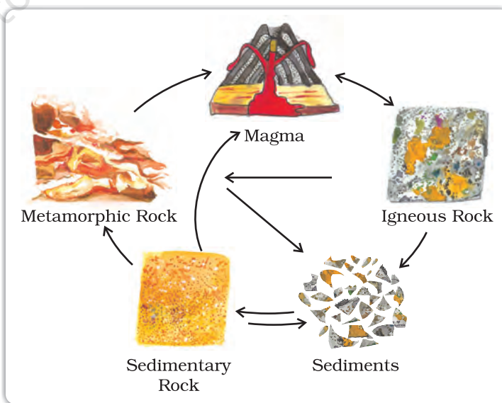
Fig. 2.4: Rock Cycle
