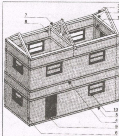
Overall arrangement of reinforcing in masonry doubly storey building having pitched roof
