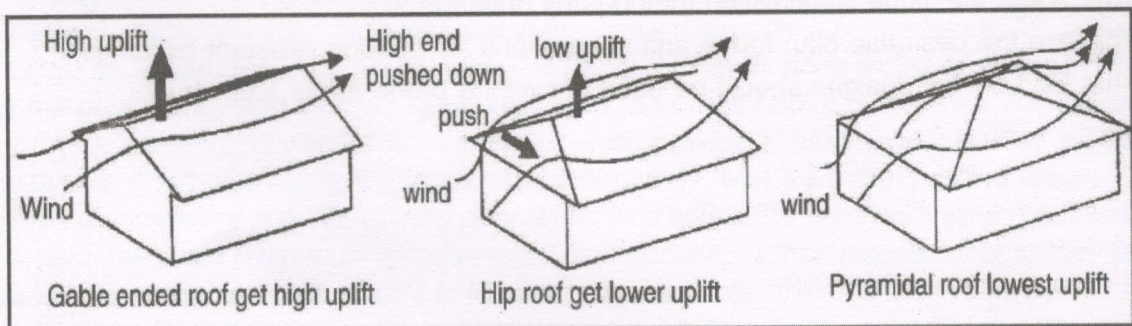
Effects of roof architecture on uplift force
