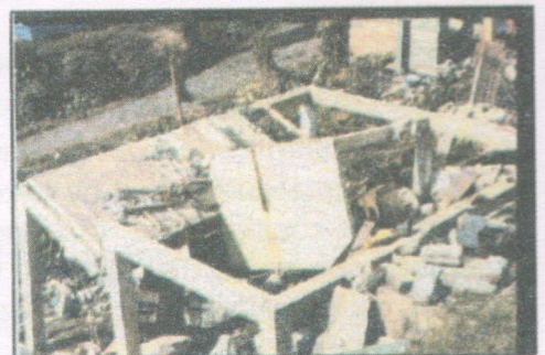
Pictures showing the effect of cyclone on structures
