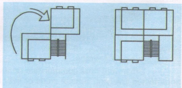
Desirable orientation & plan form for Reducing wind damage.
