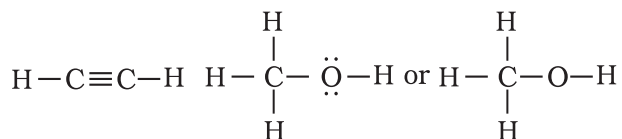
Ethyne
