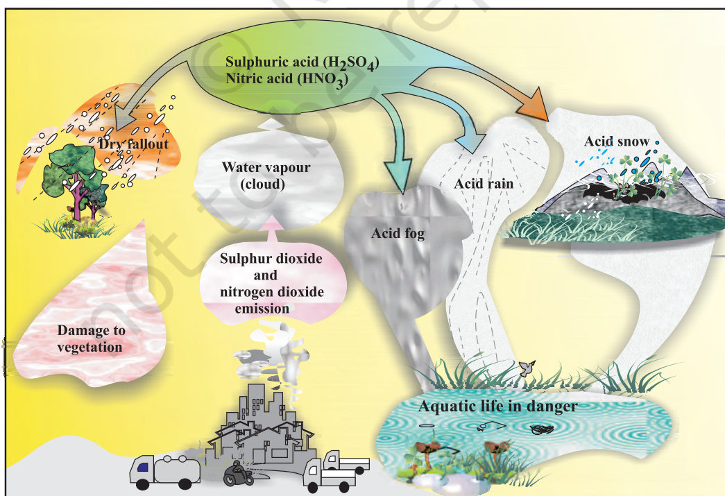
Fig. 14.1 Acid deposition
