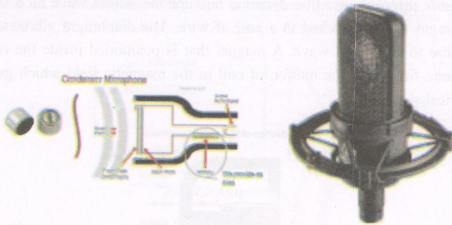
Fig. 7.5 Condenser Microphone
