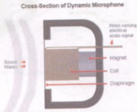
Fig. 7.4 Dynamic Microphone
