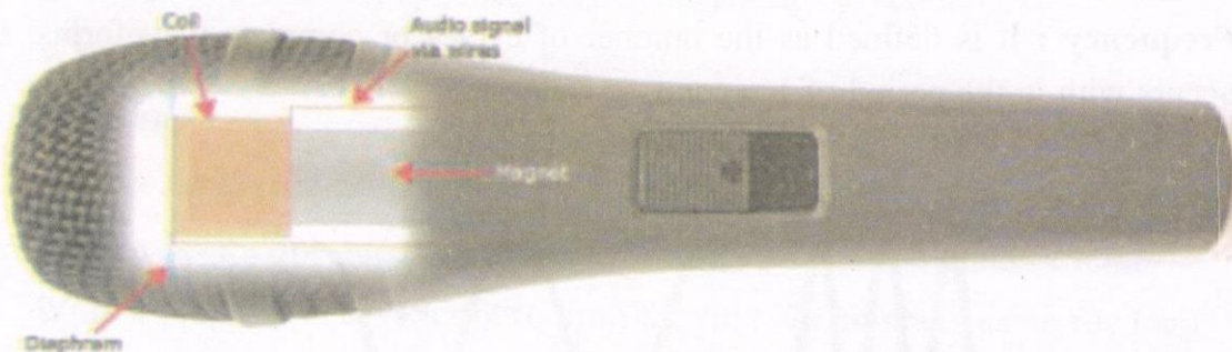
Fig. 7.3 Microphone
