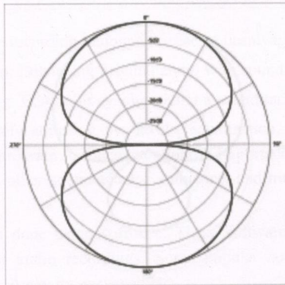
Fig. 7.8 Bi-Directional
