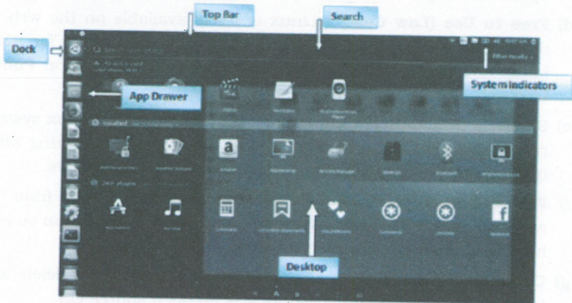
Fig. 1.7 Linux Desktop
