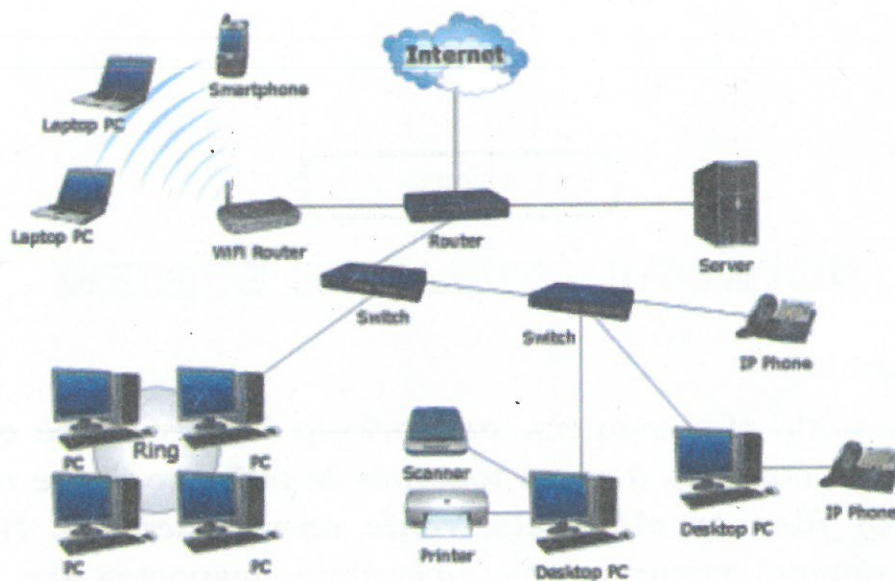
Figure 1.1 Computer Network
