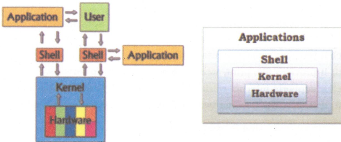
Fig. 1.5 Linux Structure
