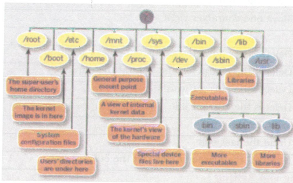
Fig. 1.9 Linux File Structure
