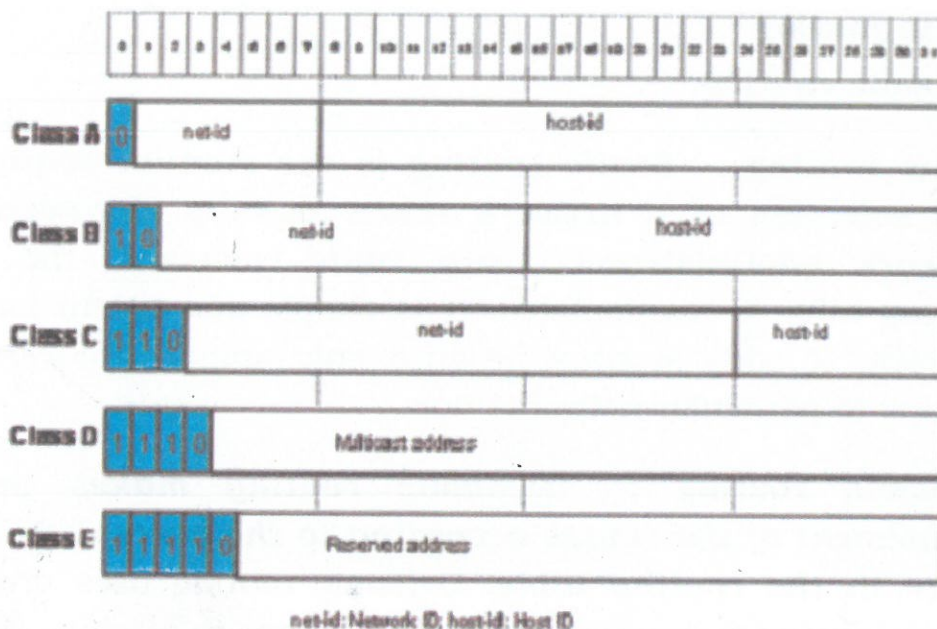
Fig. 1.3 Network ID & Host ID
