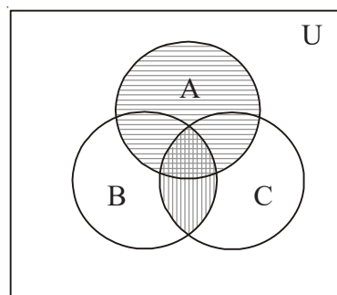
A \cup (B \cap C)
