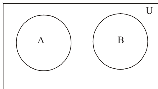
A and B are disjoint
