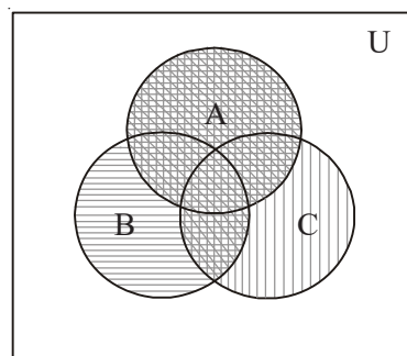
(A \cup B) \cap (A \cup C)
