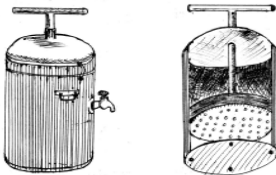
Fig. 3 : Dry cleaning pump
