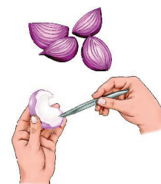
Fig. 1.3: (a) Removing onion peel from an onion bulb
