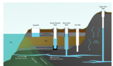
Water well types.
