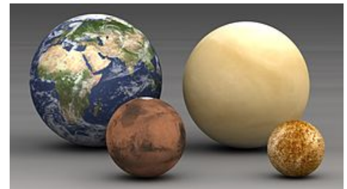
The inner planets. From left to right: Earth, Mars, Venus, and Mercury (sizes to scale).
