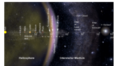
From the Sun to the nearest star: The Solar System on a logarithmic scale in astronomical units(AU)
