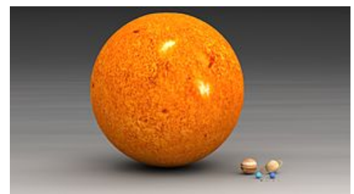
Size comparison of the Sun and the planets
