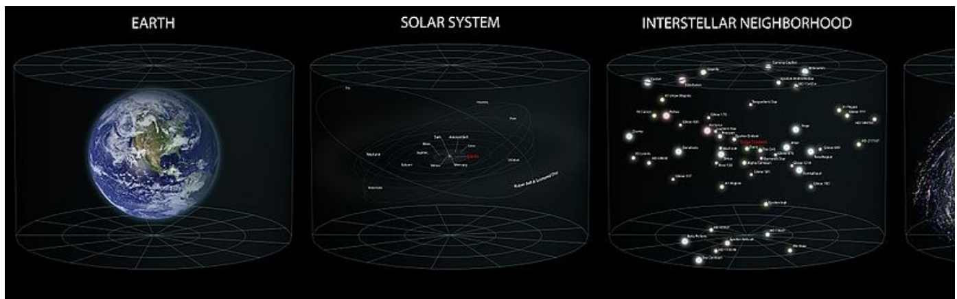
A diagram of Earth's location in the observable Universe ( Click here for an alternate image )
