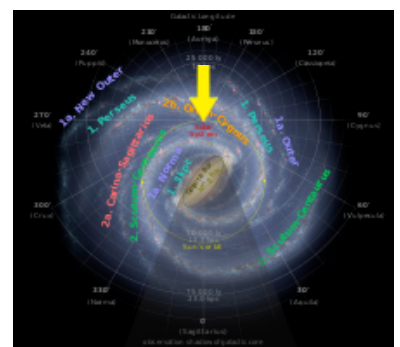
Diagram of the Milky Way with the position of the Solar System marked by a yellow arrow
