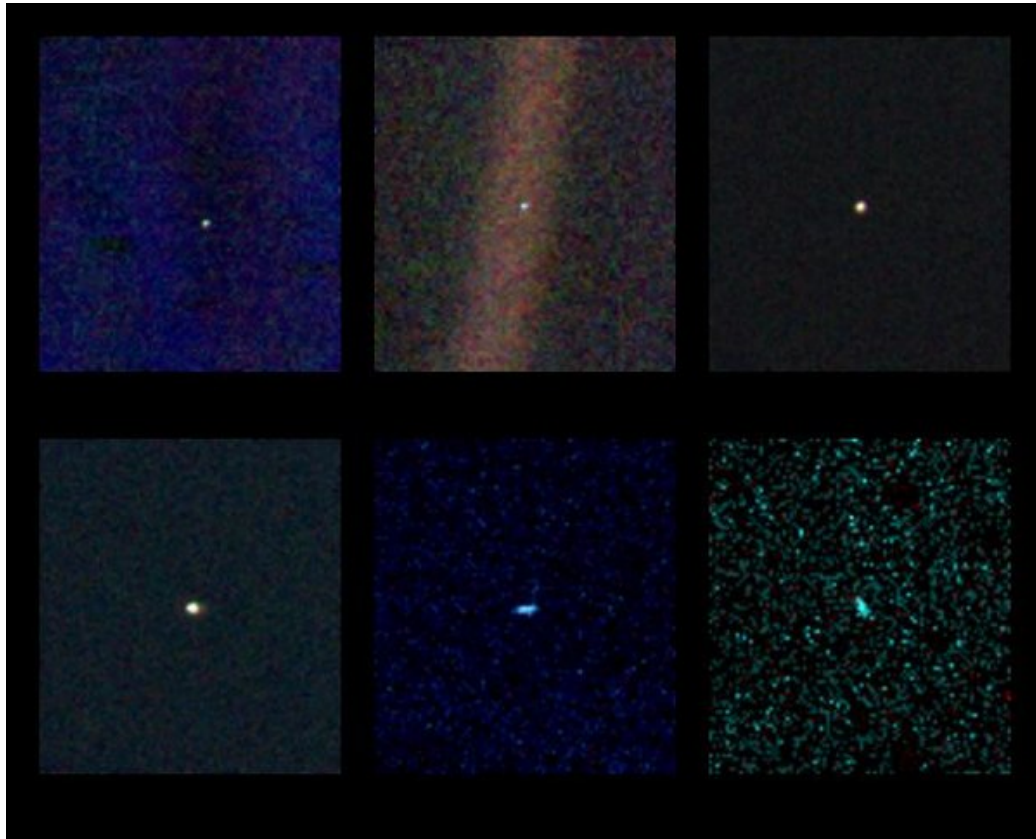
Venus, Earth ("Pale Blue Dot"), Jupiter, Saturn, Uranus, Neptune (13 September 1996).
