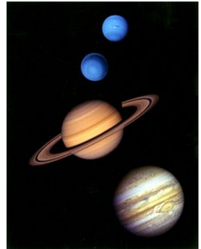
From top to bottom: Neptune, Uranus, Saturn, and Jupiter (Montage with approximate colour and relative size)
