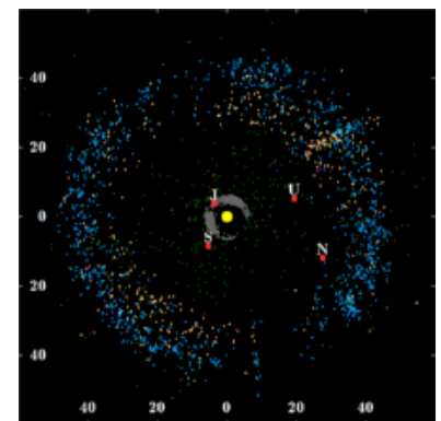
Known objects in the Kuiper belt
