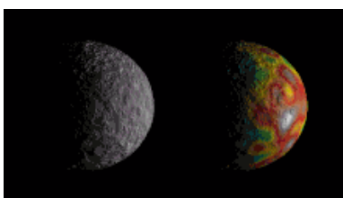
Ceres - map of gravity fields: red is high; blue, low
