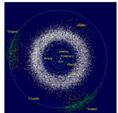
The donut-shaped asteroid belt is located between the orbits of Mars and Jupiter.
