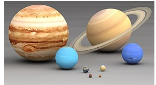
The eight planets of the Solar System (by decreasing size) are Jupiter, Saturn, Uranus, Neptune, Earth, Venus, Mars and Mercury.
