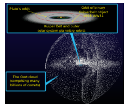
Schematic of the hypothetical Oort cloud, with a spherical outer cloud and a disc-shaped inner cloud
