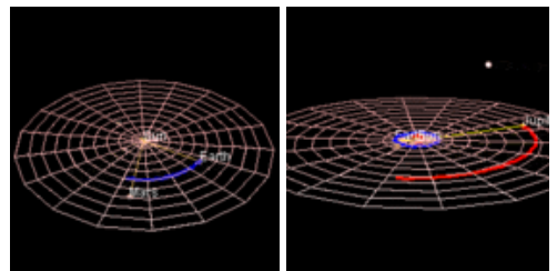
All planets of the Solar System lie very close to the ecliptic. The closer they are to the Sun, the faster they travel (inner planets on the left, all planets except Neptune on the right)
