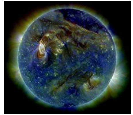
In this false-color ultraviolet image, the Sun shows a C3-class solar flare (white area on upper left), a solar tsunami (wave-like structure, upper right) and multiple filaments of plasma following a magnetic field, rising from the stellar surface.
