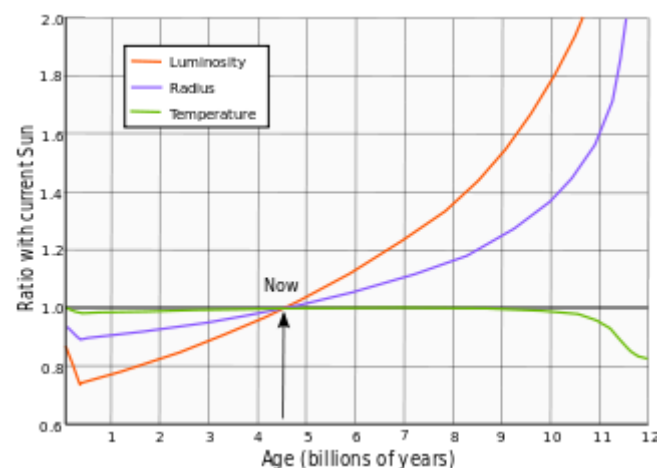
Evolution of the Sun's luminosity, radius and effective temperature compared to the present Sun. After Ribas (2010) [132]
