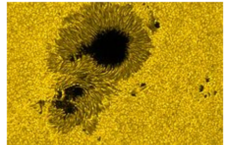
Visible light photograph of sunspot, 13 December 2006
