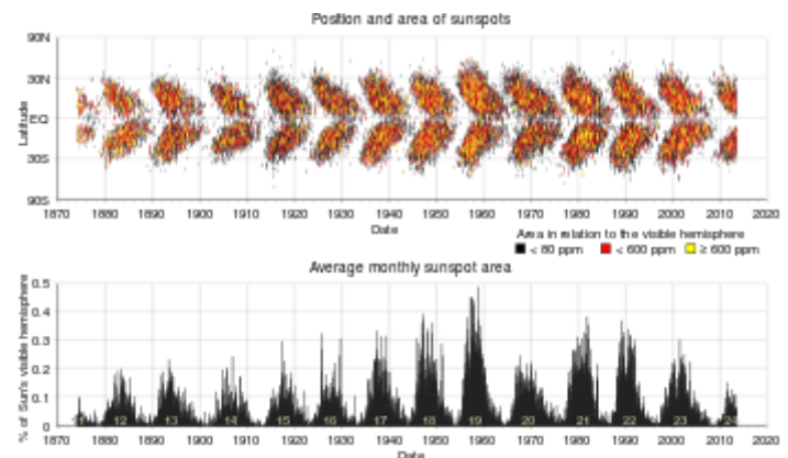
Butterfly diagram showing paired sunspot pattern. Graph is of sunspot area.
