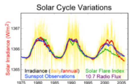
Measurements from 2005 of solar cycle variation during the last 30 years
