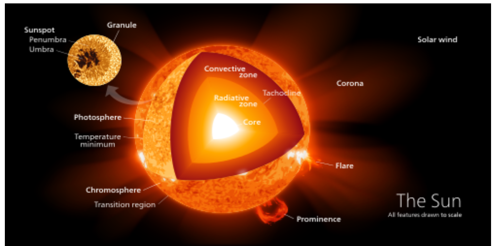
The structure of the Sun
