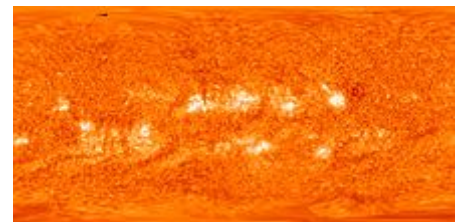
Map of the full Sun by STEREO and SDO spacecraft
