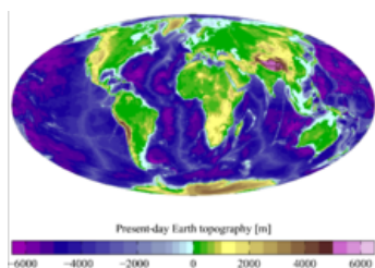
Present-day Earth altimetry and bathymetry. Data from the National Geophysical Data Center
