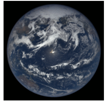
Earth's rotation imaged by DSCOVR EPIC on 29 May 2016, a few weeks before the solstice.
