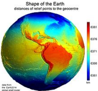
Shape of planet Earth. Shown are distances between surface relief and the geocentre. The South American Andes summits are visible as elevated areas. Data from the Earth2014 [89] global relief model.
