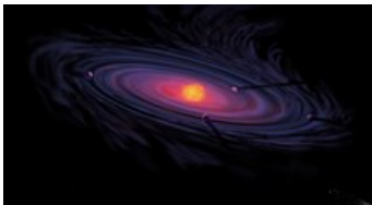
Artist's impression of the early Solar System's planetary disk
