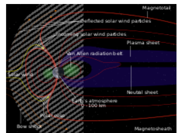
Schematic of Earth's magnetosphere. The solar wind flows from left to right
