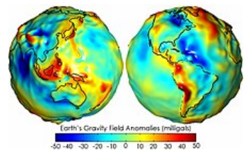
Earth's gravity measured by NASA's GRACE mission, showing deviations from the theoretical gravity. Red shows where gravity is stronger than the smooth, standard value, and blue shows where it is weaker
