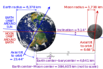
Details of the Earth–Moon system, showing the radius of each object and the Earth–Moon barycenter. The Moon's axis is located by Cassini's third law.
