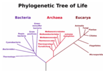
Phylogenetic tree of life on Earth based on rRNA analysis
