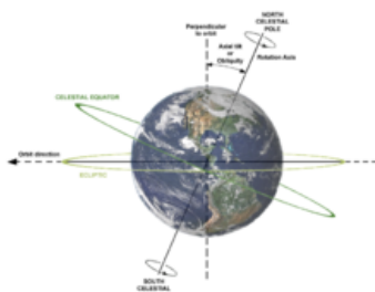
Earth's axial tilt (obliquity) and its relation to the rotation axis and plane of orbit
