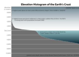
Elevation histogram of Earth's surface
