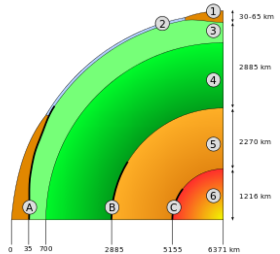
Schematic view of the interior of Earth. 1. continental crust – 2. oceanic crust – 3. upper mantle – 4. lower mantle – 5. outer core – 6. inner core – A: Mohorovičić discontinuity – B: Gutenberg Discontinuity – C: Lehmann–Bullen discontinuity
