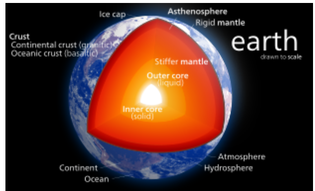
Structure of the Earth
