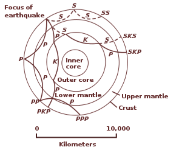
Mapping the interior of Earth with earthquake waves.
