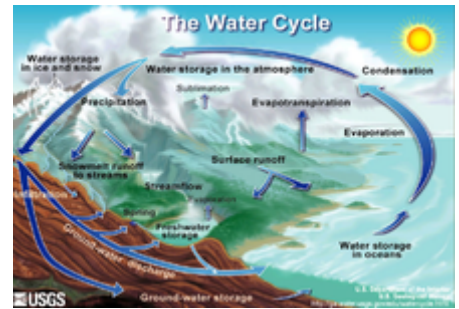
Water cycle
