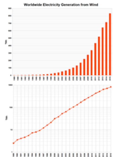
Worldwide wind generation up to 2012 [57]
