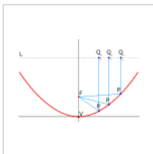
A parabolic mirror brings parallel rays of light to a focus.
