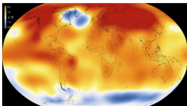
2015 – Warmest Global Year on Record (since 1880) – Colors indicate temperature anomalies (NASA/NOAA; 20 January 2016) [9]
