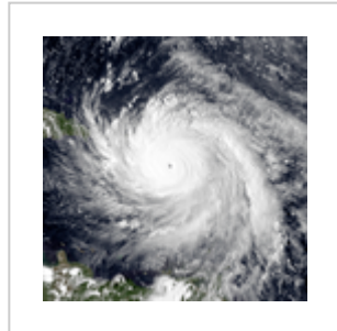
Atlantic hurricane
