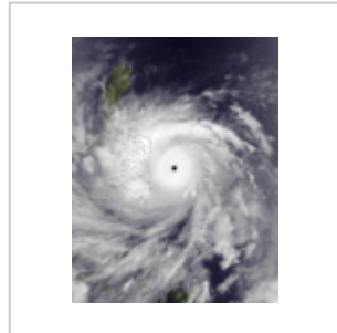
Pacific typhoon
