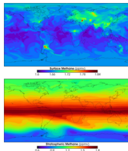
Global methane concentrations (surface and atmospheric) for 2005; note distinct plumes
