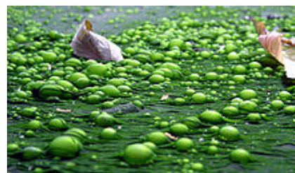
An algal bloom caused by eutrophication
