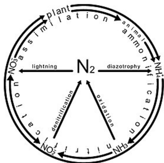
Classical representation of nitrogen cycle
