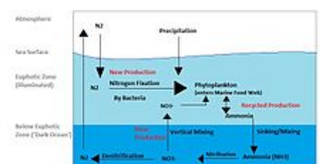
A schematic representing the Marine Nitrogen Cycle
