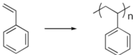
Styrene polymerization
