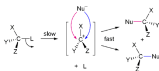
S N 1 mechanism
