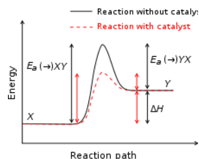
Schematic potential energy diagram showing the effect of a catalyst in an endothermic chemical reaction. The presence of a catalyst opens a different reaction pathway (in red) with a lower activation energy. The final result and the overall thermodynamics are the same.
