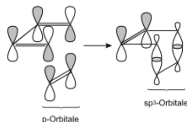
Orbital overlap in a Diels-Alder reaction
