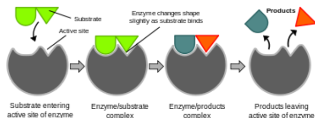
Illustration of the induced fit model of enzyme activity
