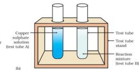
Figure 1.8 (b) Iron nails and copper sulphate solutions compared before and after the experiment
