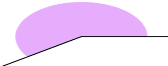
Reflex Angle
